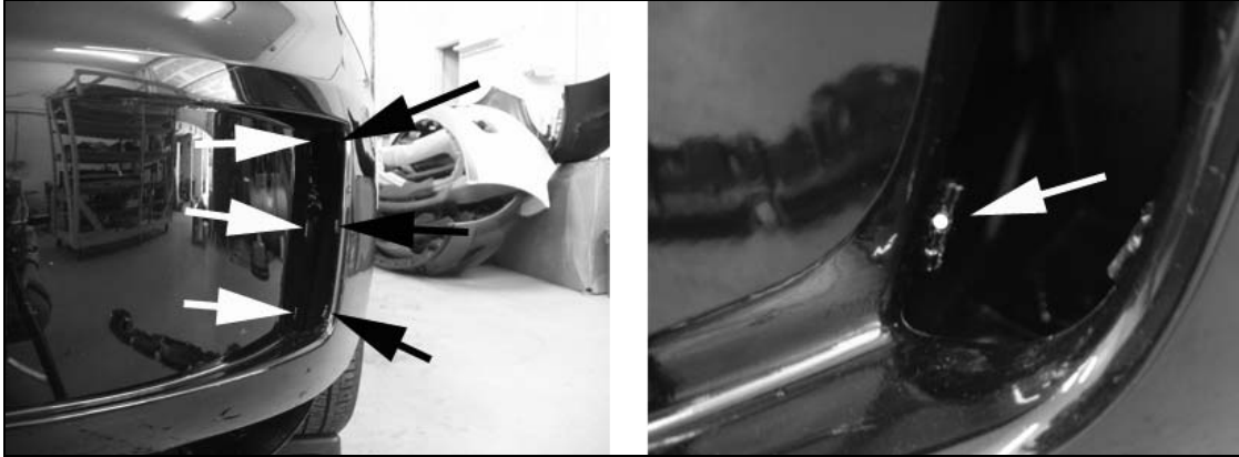
Figure 6. Drille the 1/8" holes in the locations shown.
