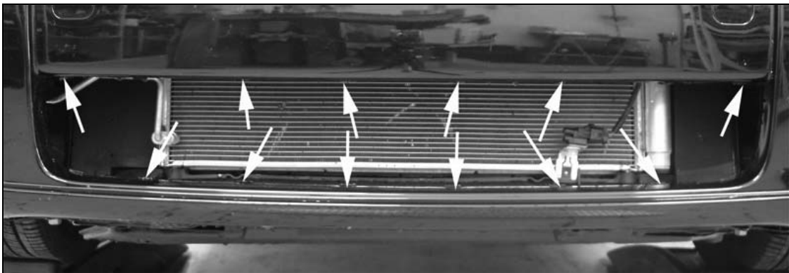
Figure 3. Drille 1/8" holes in the tabs at these locations.
