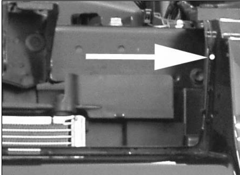
Figure 2. Drill a 1/8" hole on each side of the upper grille opening in this location.
