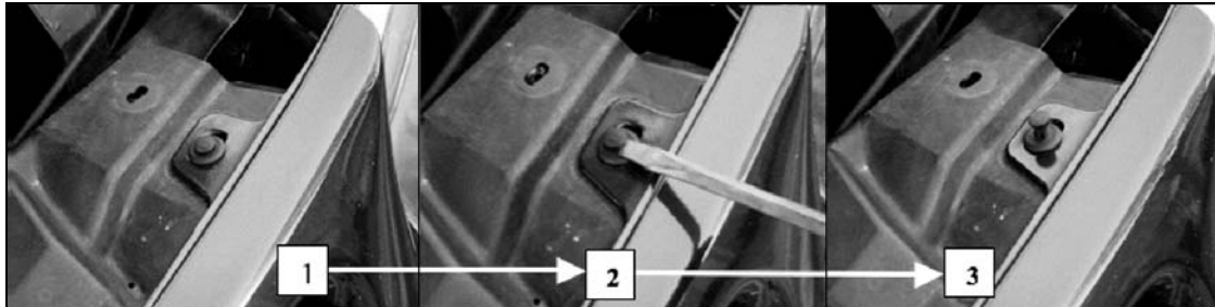
Figure 1. Procedure for removing a pop-top fastener.
